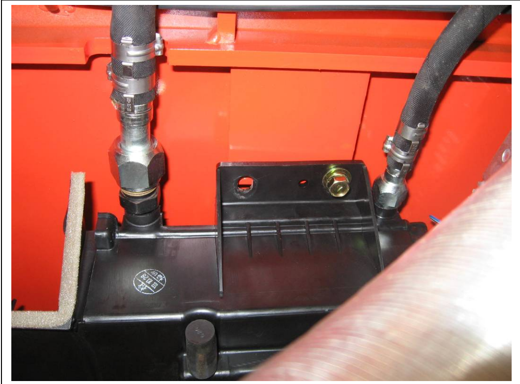
Evap reinstalled and hoses connected.
